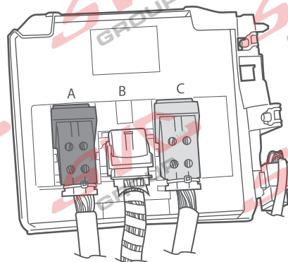
Body Control Module
